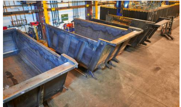
Tipper body sub-frames for three-way tippers, tipper bodies for rectangular rear tippers and half-pipe tipper bodies for rear tippers and semitrailers are produced with the robot system.
